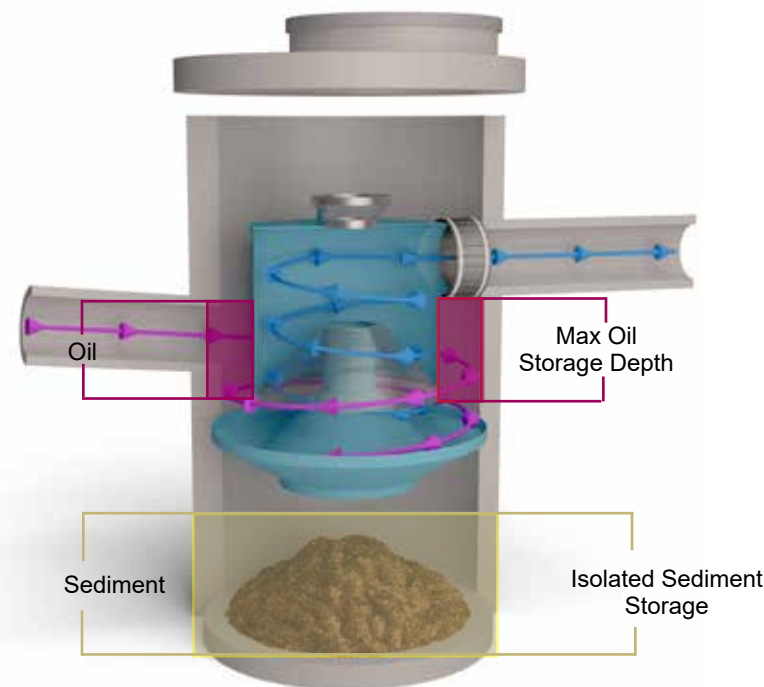
Fig.1 Pollutant storage volumes of the Downstream Defender®.
