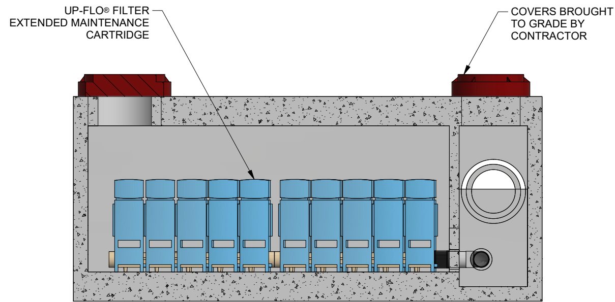
SECTION A-A ELEVATION VIEW
