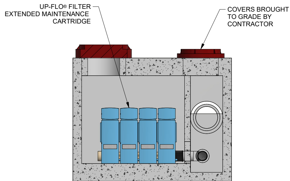
SECTION A-A ELEVATION VIEW
